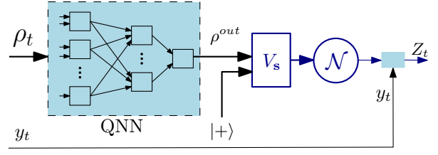
Figure 2: The procedure for measuring the derivative of the loss consisting of a unitary operator V_s followed by a quantum measurement \mathcal{N} with additional classical processing.
